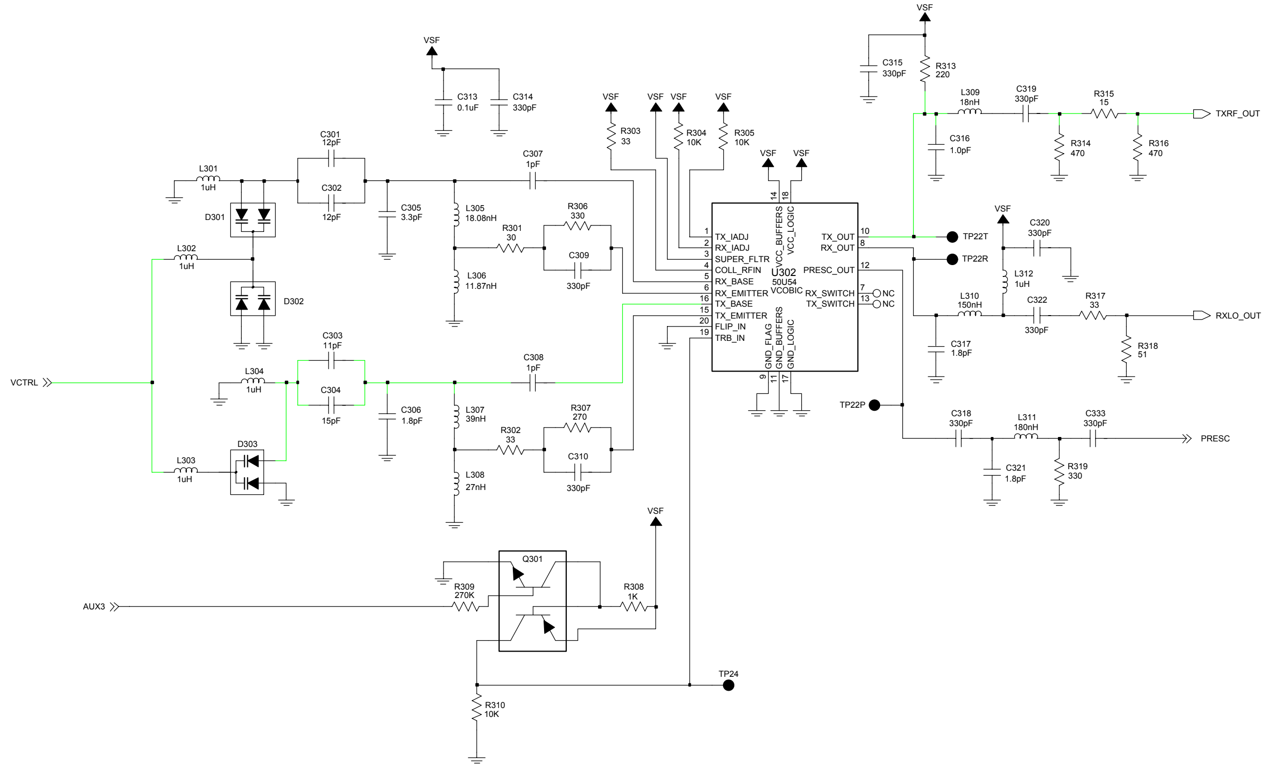
Figure 8-28. NLD8910B VHF Frequency Generation Unit (VCO) Circuit
