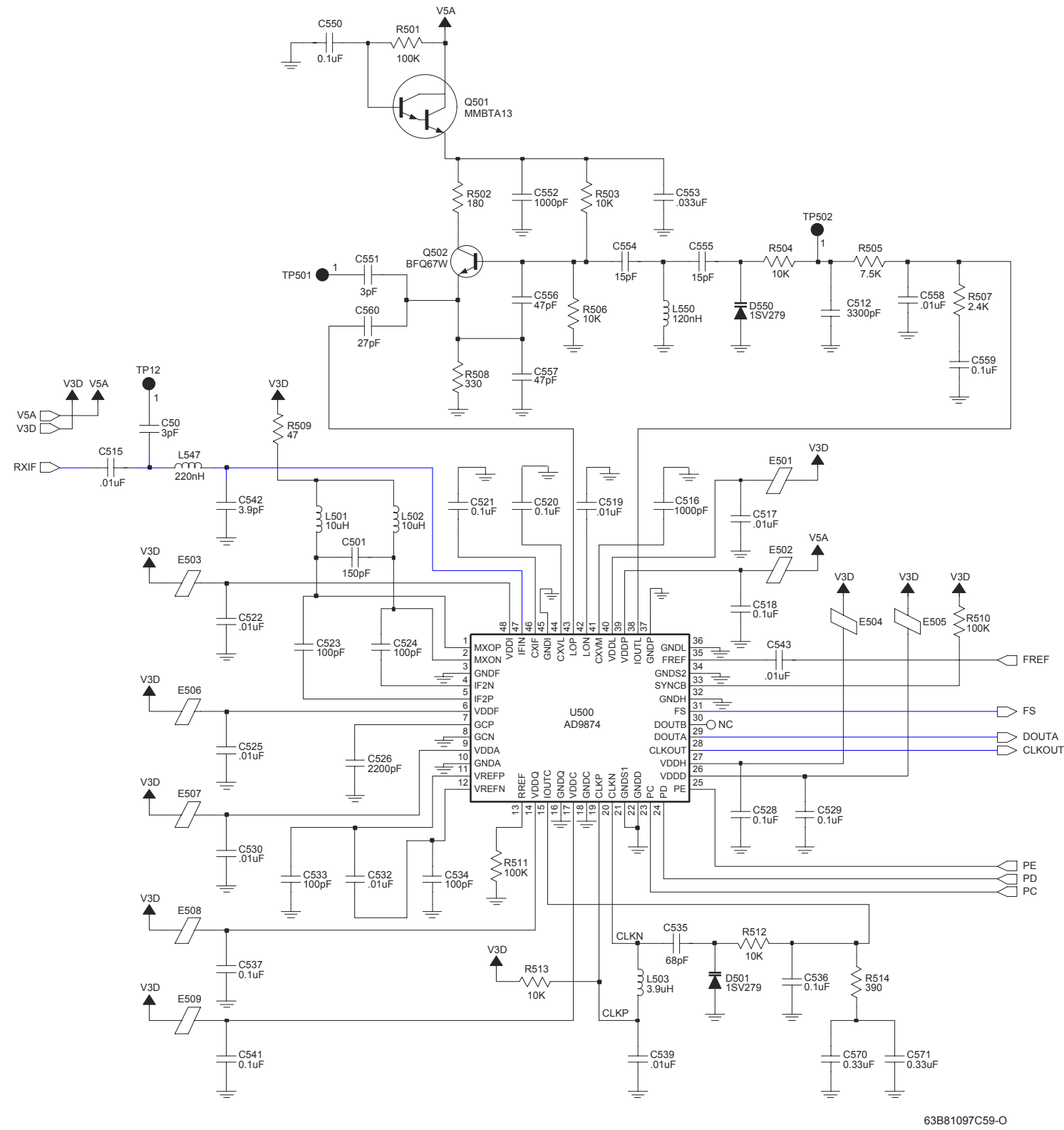
Figure 8-13. NUF3577C 700–800 MHz Receiver Back End Circuit
