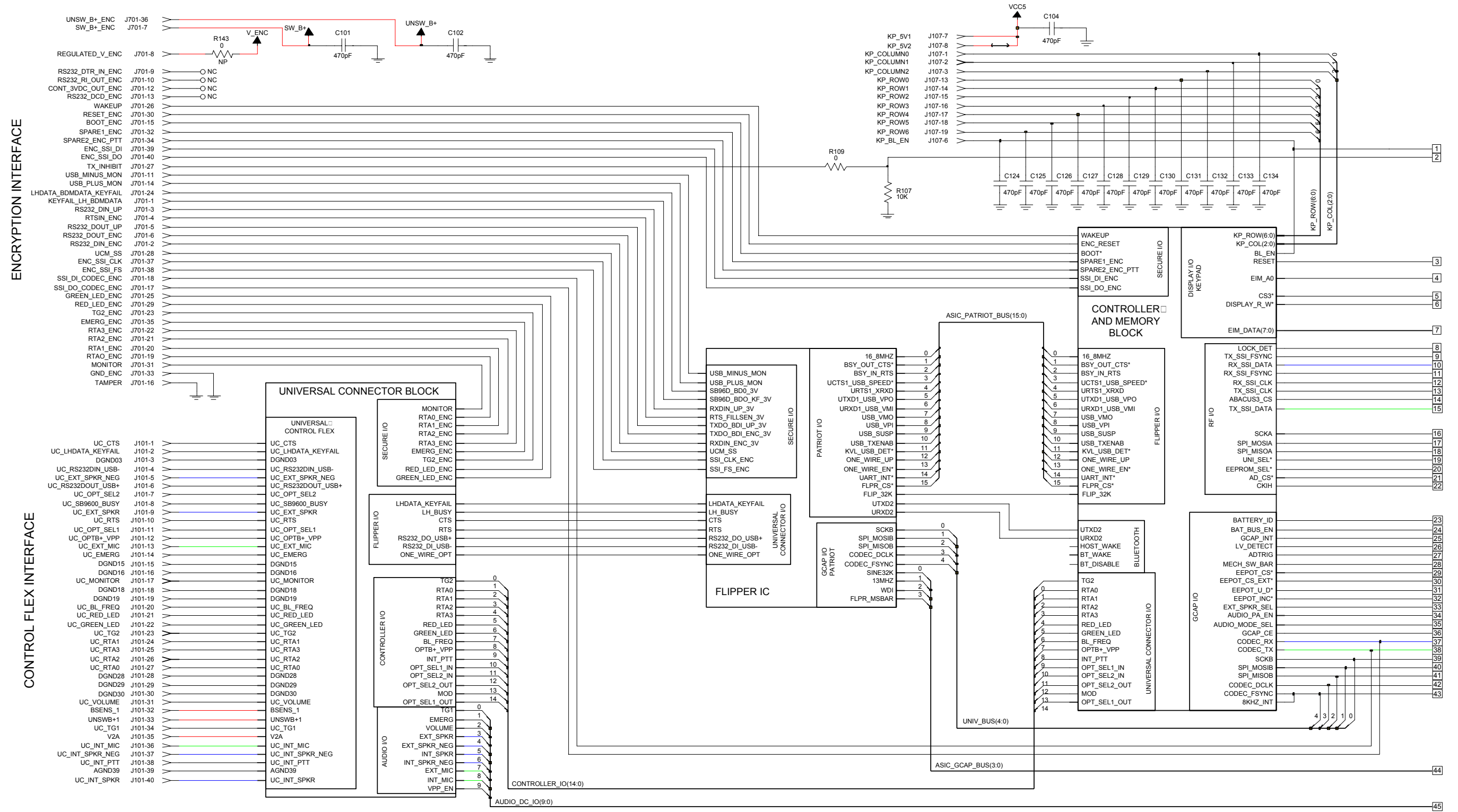
Figure 8-70. NTN9564C VOCON Board Overall Schematic—1 of 2
