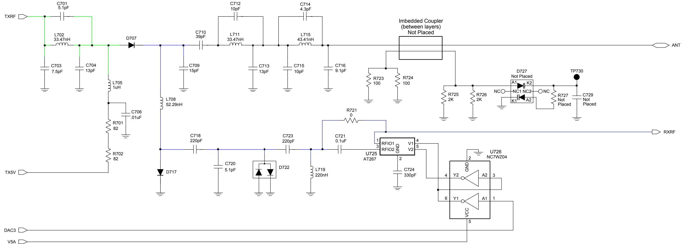
Figure 8-21. NLD8910B VHF Antenna Switch and Harmonic Filter Circuits
