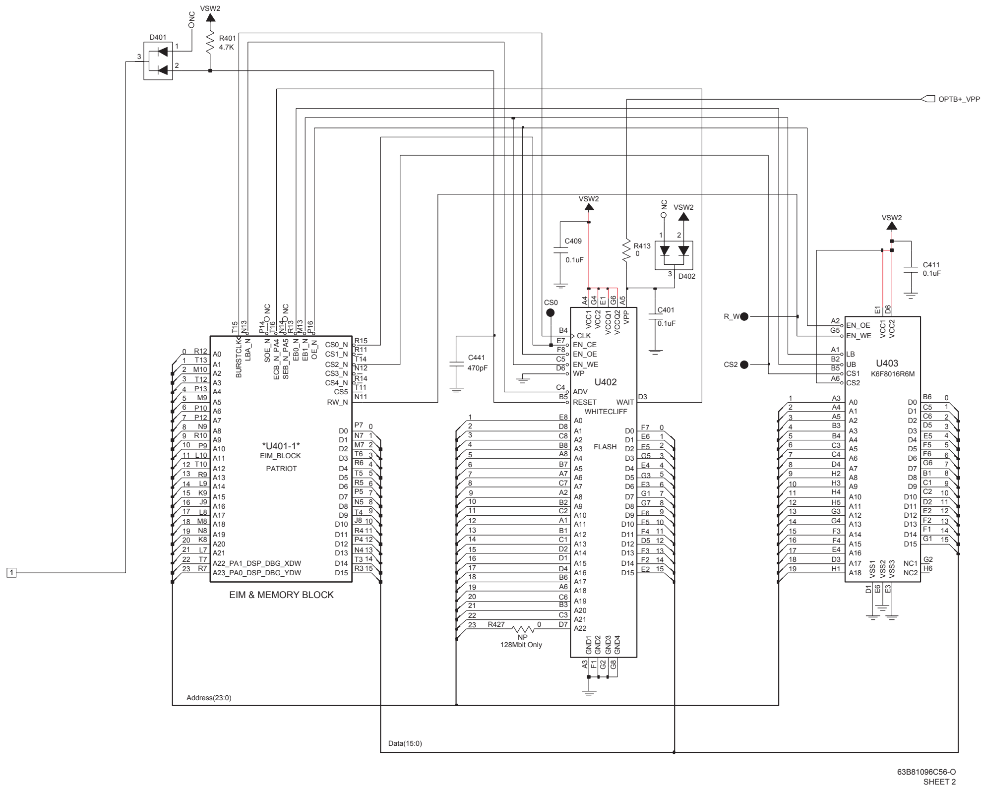
Figure 8-84. NNTN4563A/B VOCON Controller and Memory Circuits—2 of 2
