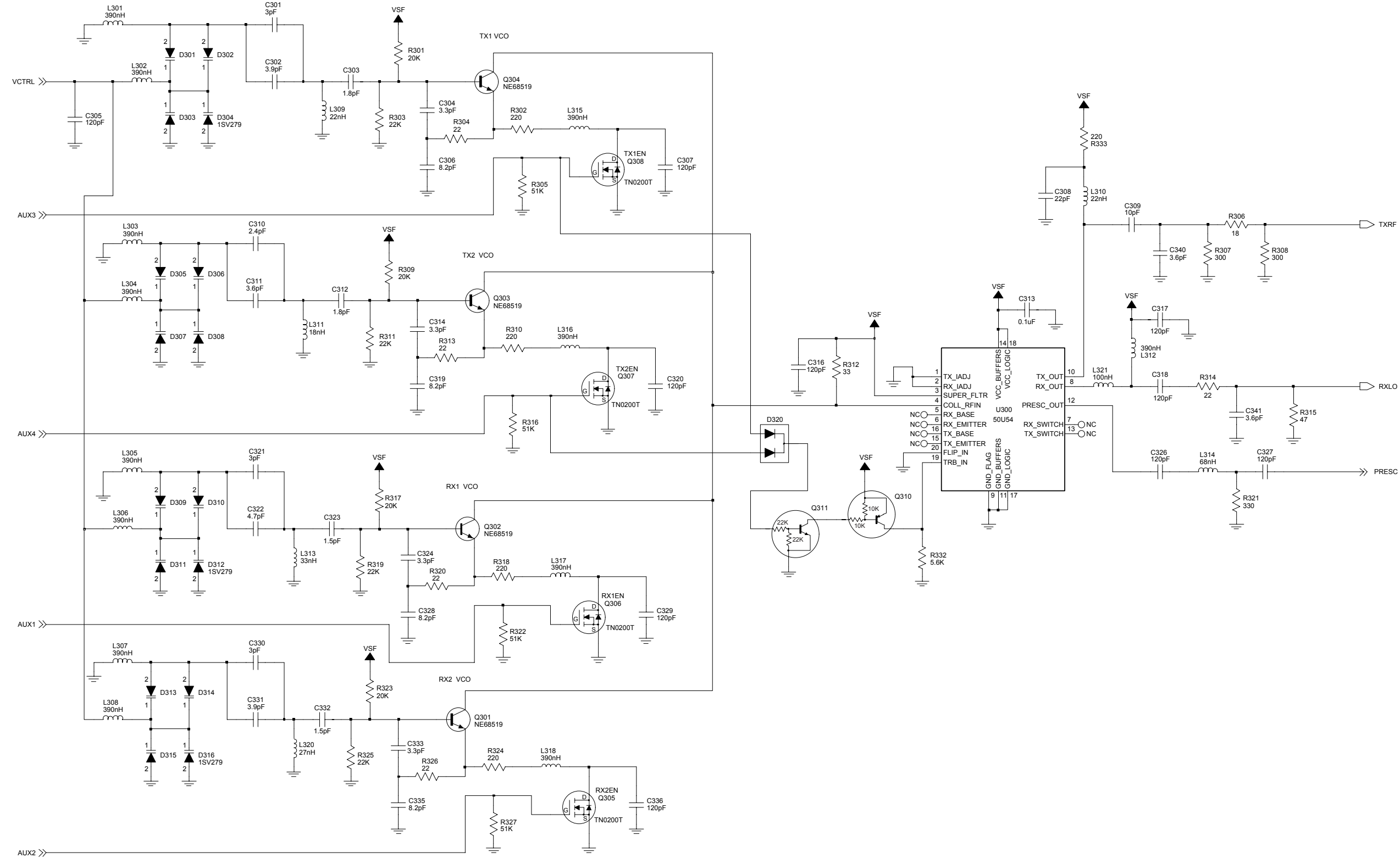
Figure 8-37. NLE4272A UHF Range 1 Frequency Generation Unit (VCO) Circuit
