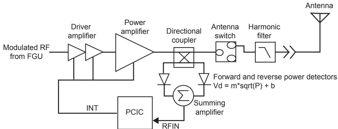
Figure 3-6. Transmitter Block Diagram
