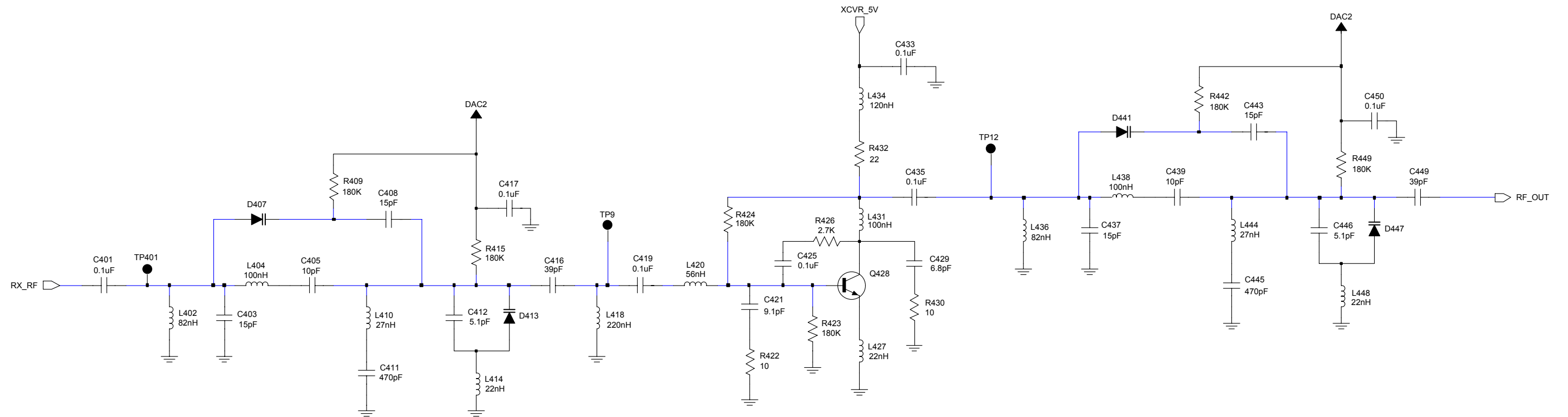
Figure 8-23. NLD8910B VHF Receiver Amplifier and Filter Circuit
