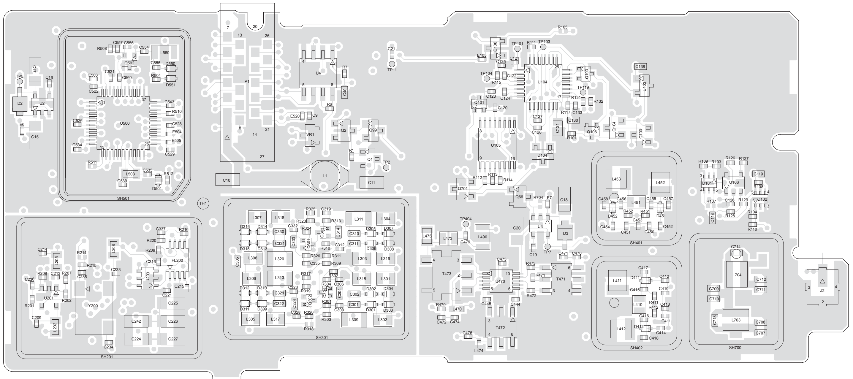
Figure 8-38. NLE4272A UHF Range 1 Transceiver (RF) Board Layout—Side 1
