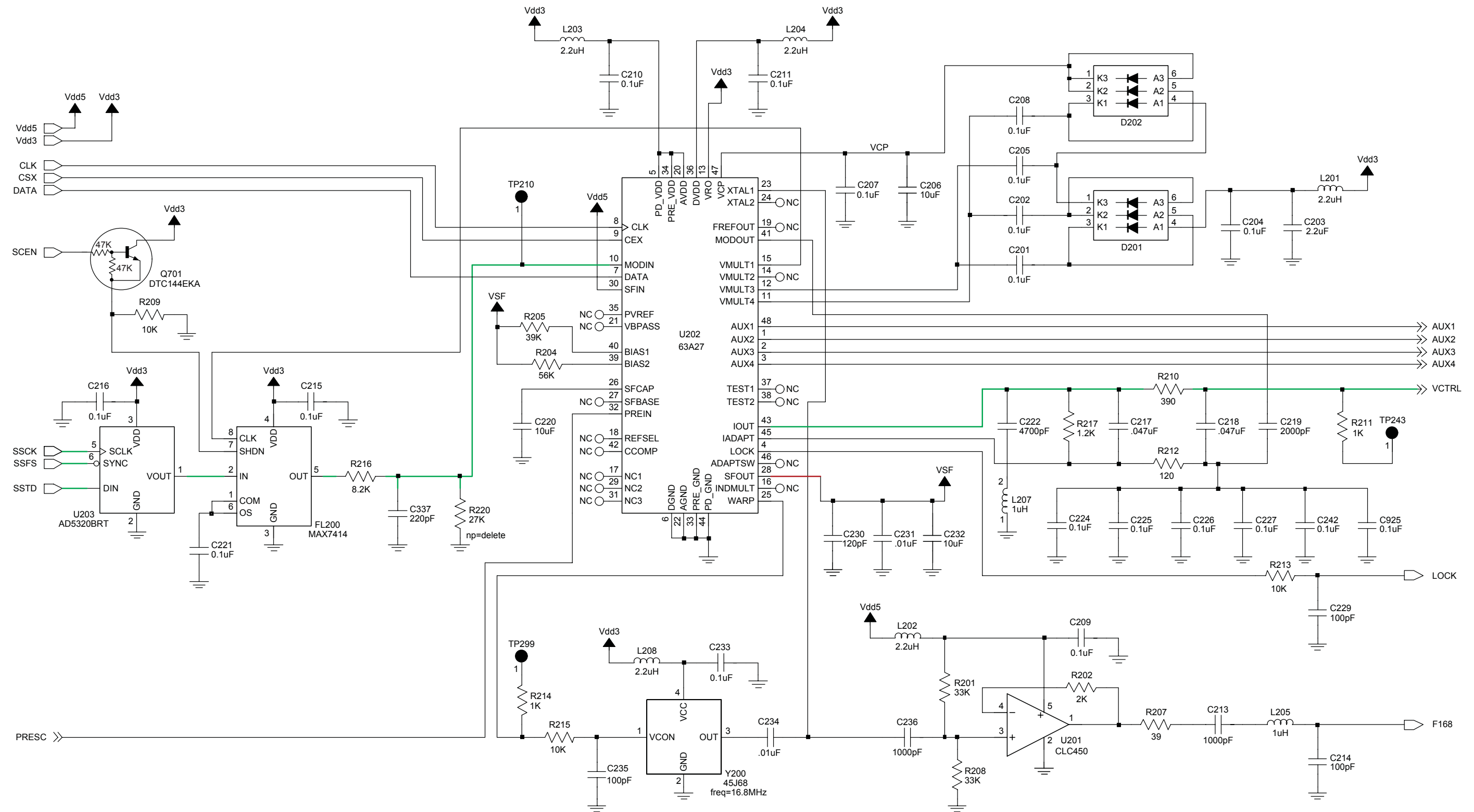
Figure 8-36. NLE4272A UHF Range 1 Frequency Generation Unit (Synthesizer) Circuit
