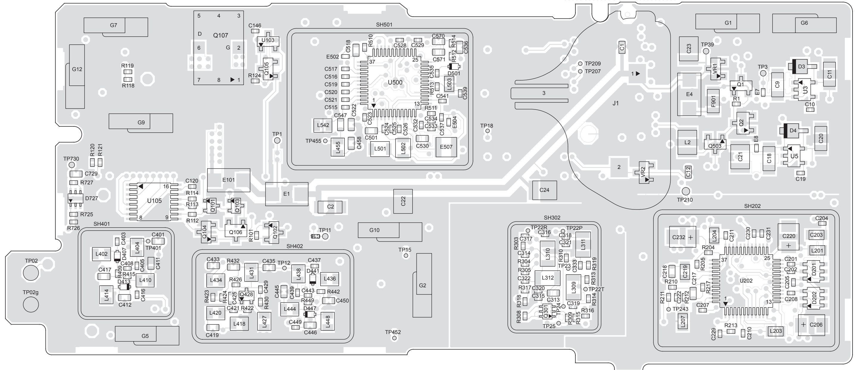
Figure 8-30. NLD8910B VHF Transceiver (RF) Board Layout—Side 2
