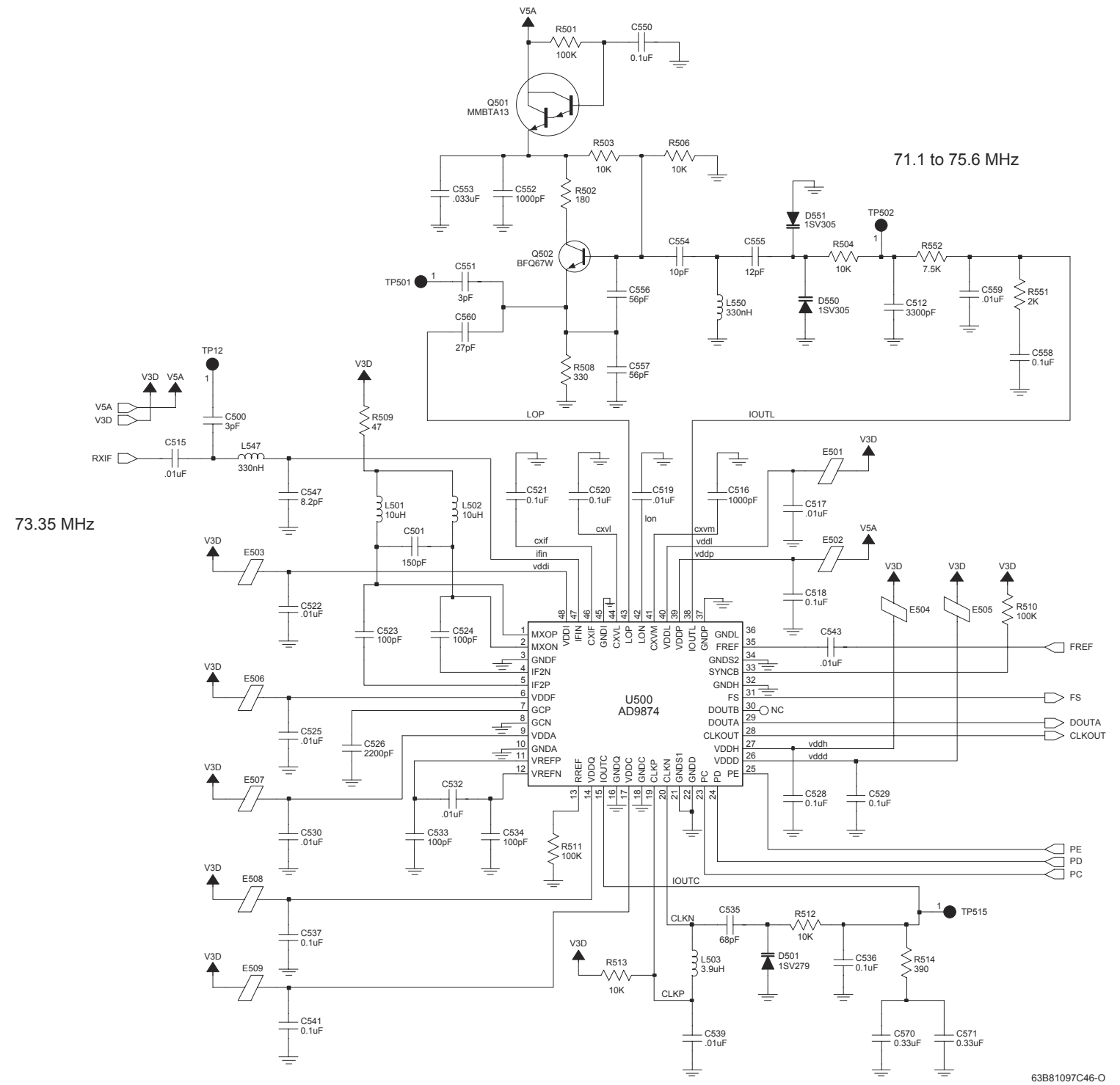
Figure 8-43. NLE4278A UHF Range 1 Receiver Back End Circuit
