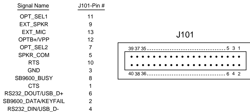
Figure 3-10. VOCON Board Connector—J101
