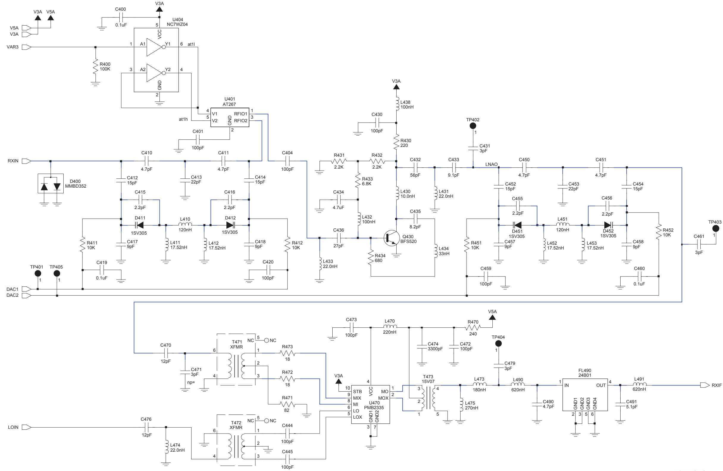
Figure 8-33. NLE4272A UHF Range 1 Receiver Front End (RX_FE) Circuit
