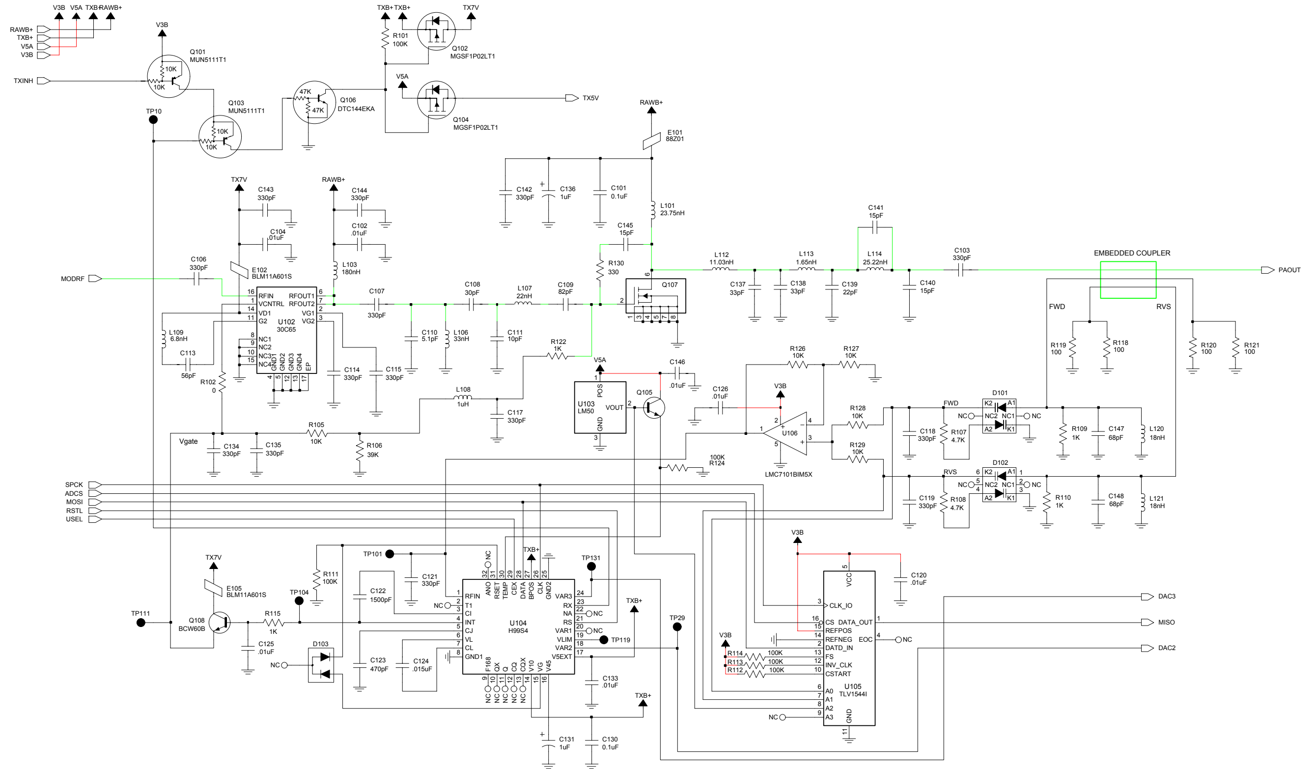
Figure 8-26. NLD8910B VHF Transmitter and Automatic Level Control Circuits
