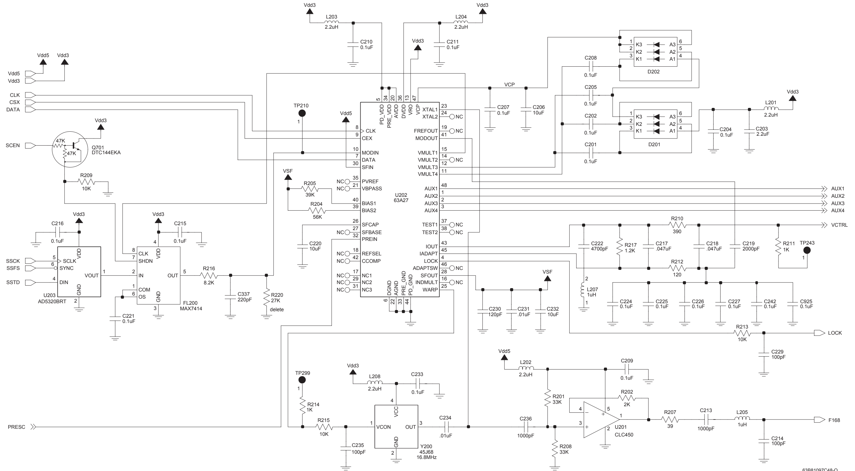
Figure 8-45. NLE4278A UHF Range 1 Frequency Unit (Synthesizer) Circuit
