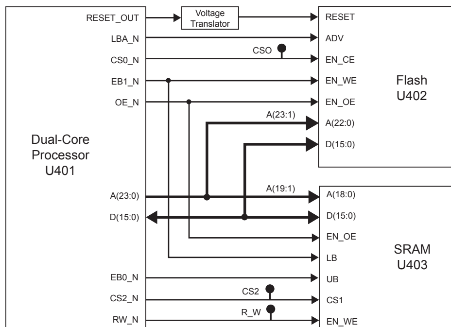
Figure 3-8. Patriot EIM and Memory Block Diagram
