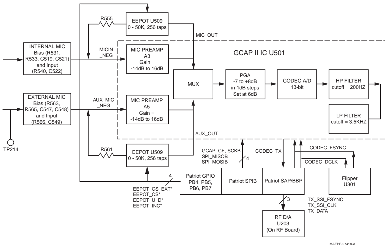
Figure 3-12. VOCON Transmit Audio Path
