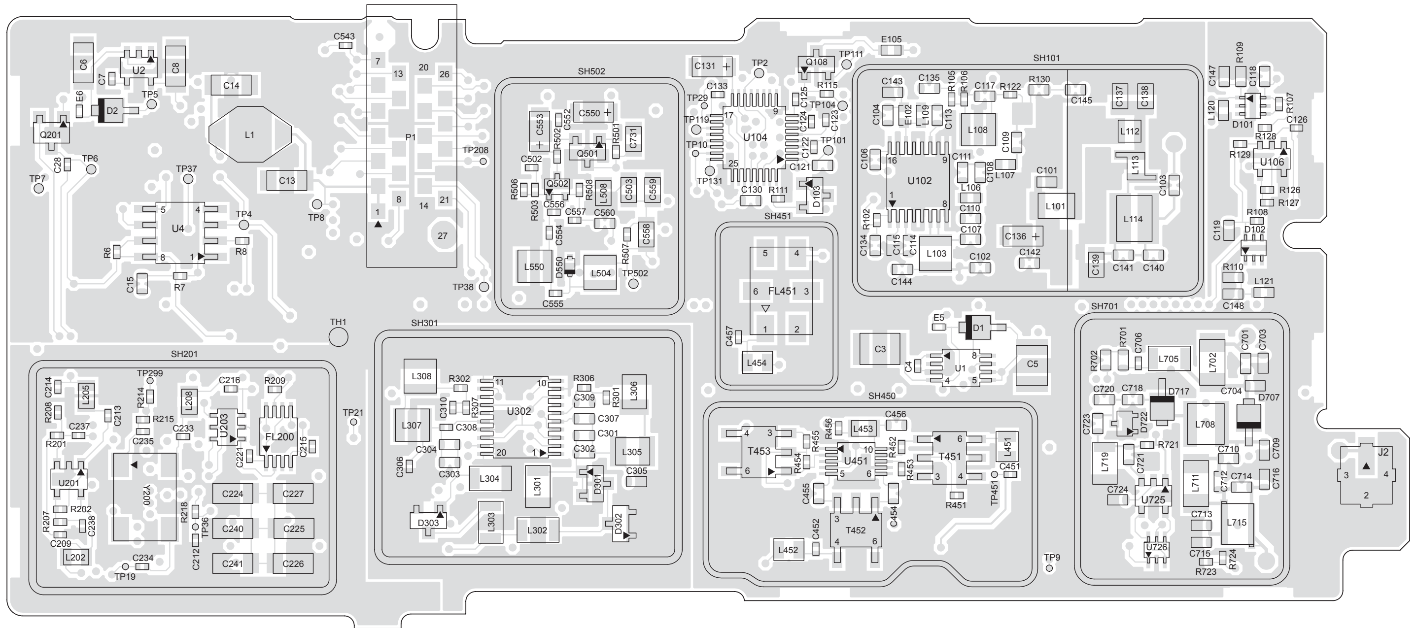
Figure 8-29. NLD8910B VHF Transceiver (RF) Board Layout—Side 1
